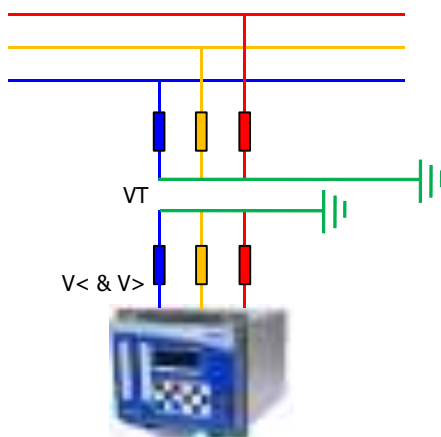
Under & Over voltage detection through 3-phase VT connection
