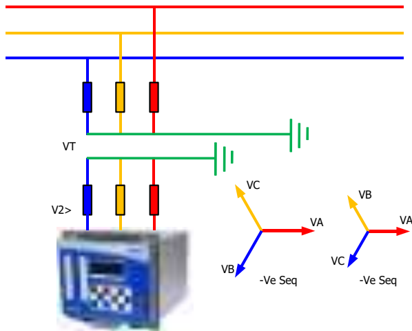
Positive/Negative Phase Sequence Over voltage detection through 3-phase VT connection
