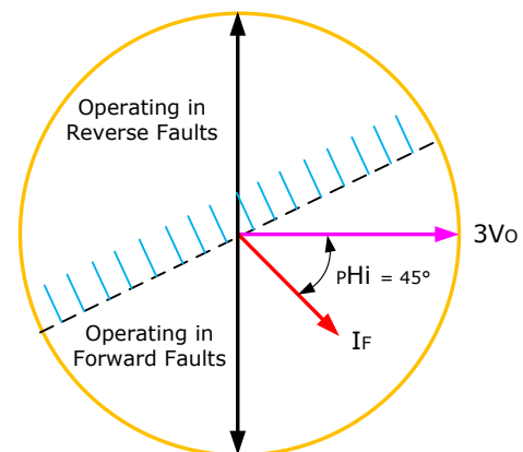
Directional discrimination for phase to ground fault
