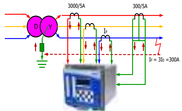
Externally measured ground over current through CBCT
