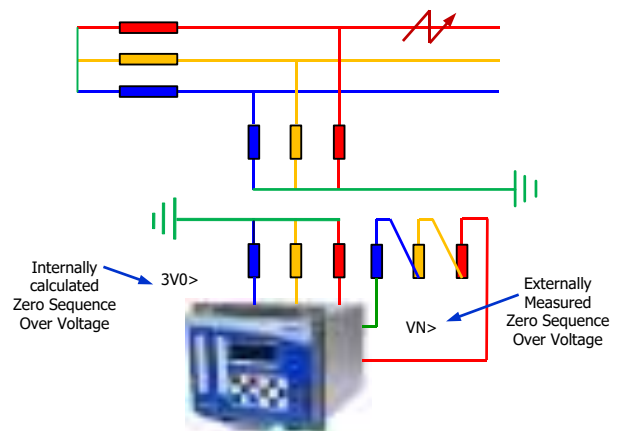
Zero sequence Over voltage / Externally measured residual Over Voltage detection through 3-phase VT & Open delta VT connections
