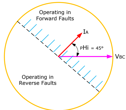
Directional discrimination for phase to phase fault
