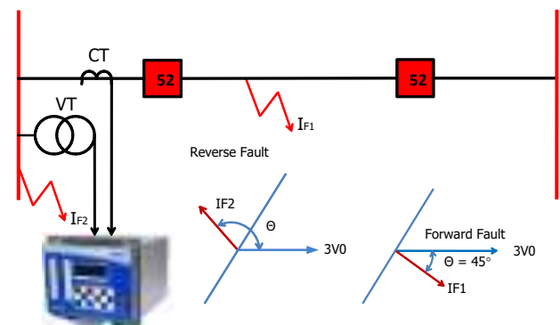
Directional determination for Ground faults
